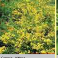
Cassia biflora
